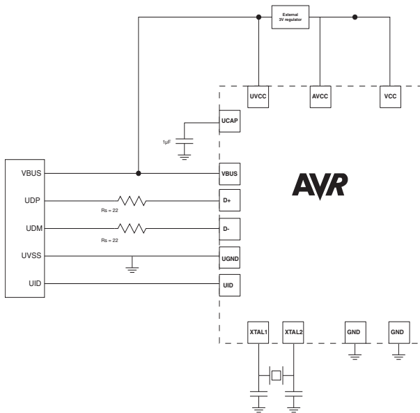
Figure 22-4. Typical bus powered application with 3V I/O.
