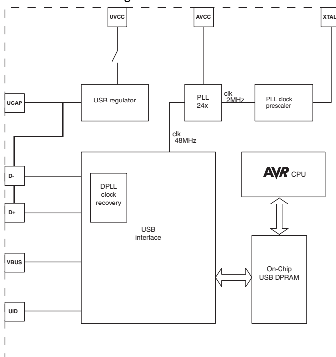
Figure 22-1. USB controller block diagram overview.
