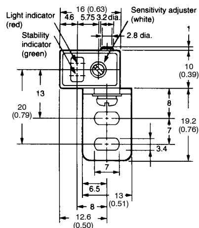
Receiver
