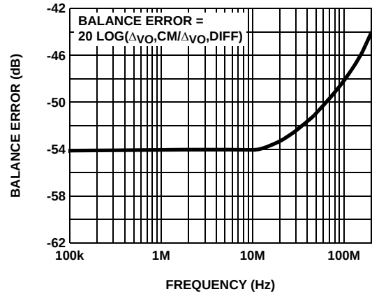
FIGURE 2. BALANCE ERROR
