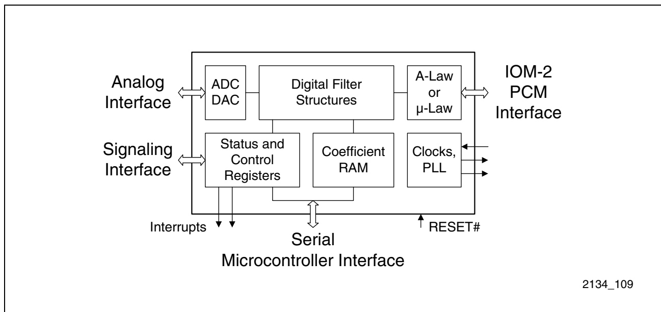
Figure 6 SICOFI®4-TE Interfaces
