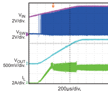
Start up through IN I_{OUT} = 3A(CC\text{-}Load)
