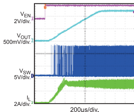
Start up through EN I_{OUT} = 3A(CC\text{-}Load)
