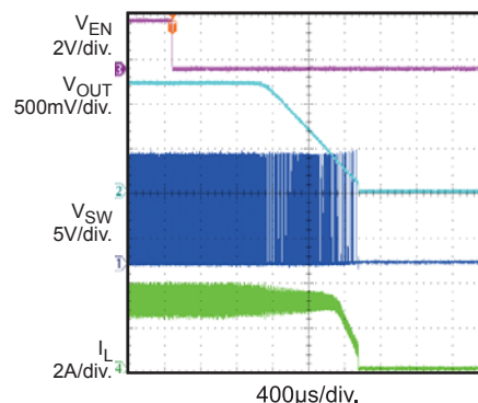
Power down through EN I_{OUT} = 3A(CC\text{-}Load)
