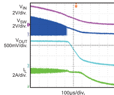
Power down through IN I_{OUT} = 3A(CC\text{-}Load)
