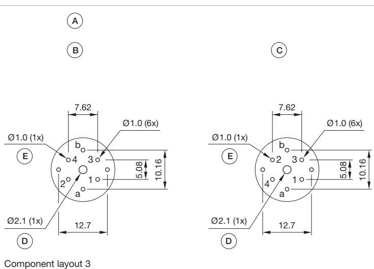
Component layout 3
