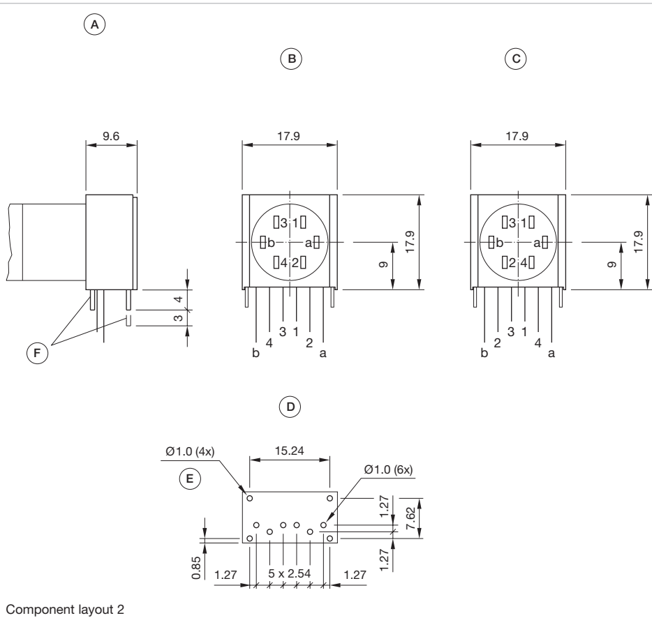
Component layout 2
