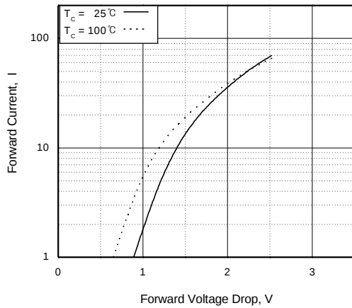
Fig 18. Forward Characteristics
