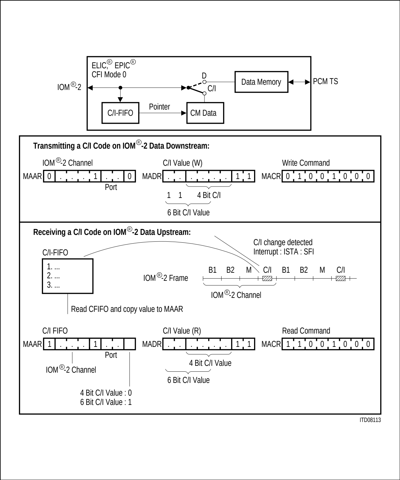
Figure 149 Receiving and Transmitting IOM ® -2 C/I-Codes (working sheet)
