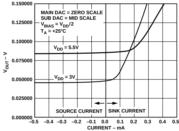
Figure 29. Sink and Source Current with Zero Scale Loaded to DAC. V_{DD} = 5V and V_{DD} = 3V
