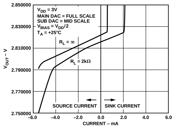
Figure 31. Sink and Source Current at Full Scale with V_{DD} = 3V
