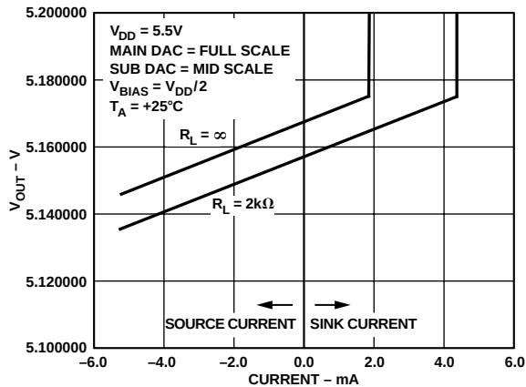
Figure 30. Sink and Source Current at Full Scale with V_{DD} = 5V
