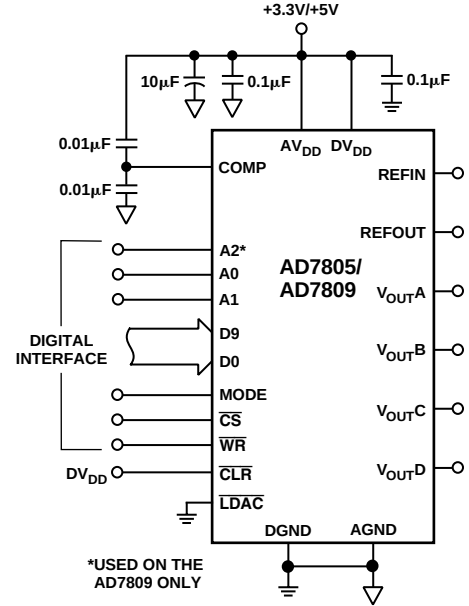
Figure 24. Typical Configuration for AD7805/AD7809
