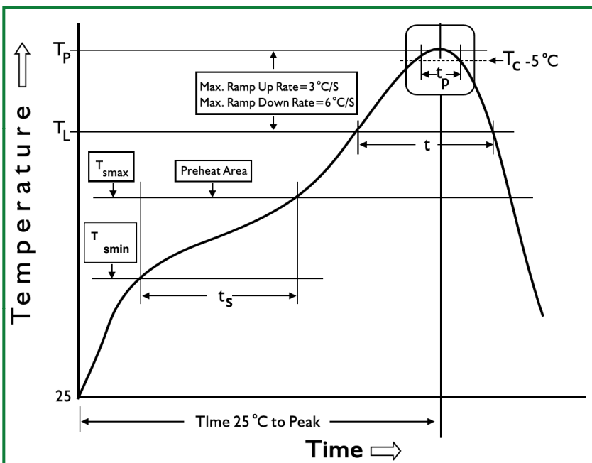
Lead-Free IR Reflow Profile (IPC/JEDEC J-STD-020D)
