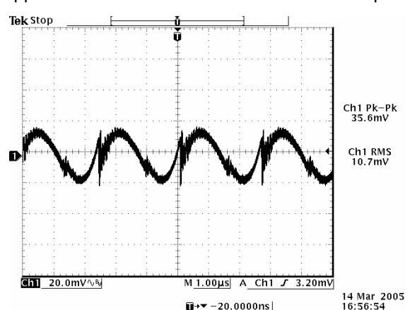
Ripple and noise at max load 1.5 Vdc/30 A output
