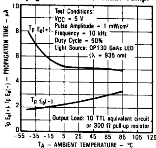
Propagation Time vs. Amb. Temp.
