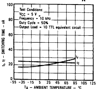
Rise Time & Fall Time vs. TA
