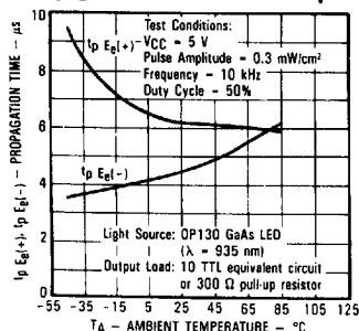
Propagation Time vs. Amb. Temp.
