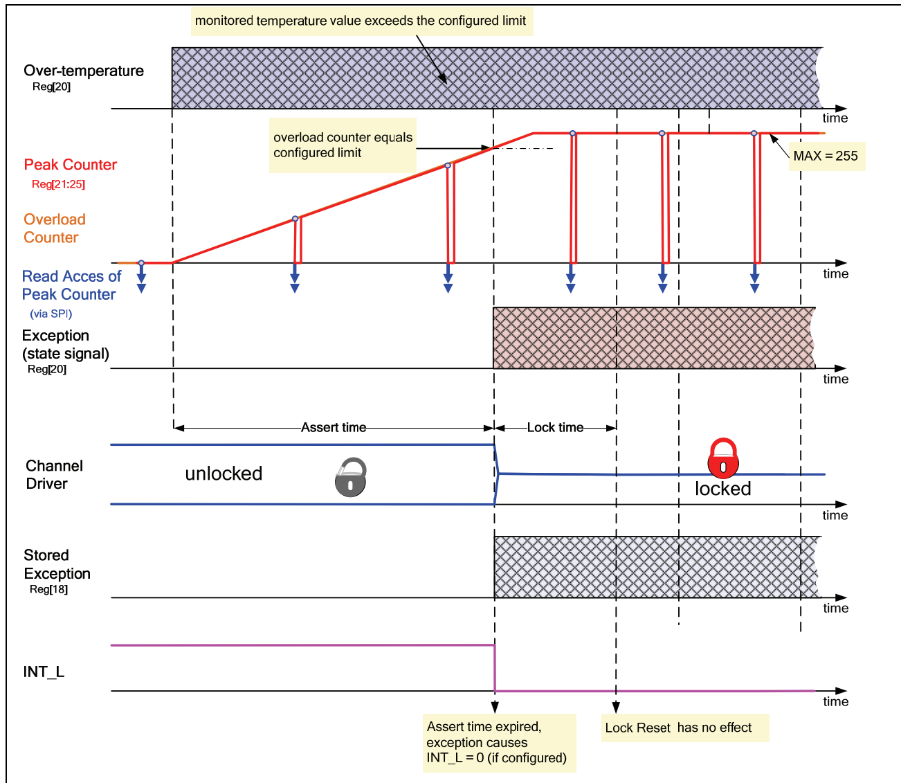
Figure 10.3 Overload Counter Behavior in permanent Over-Temperature Situations
