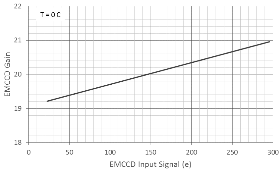
Figure 25. EMCCD Gain vs. Input Signal
