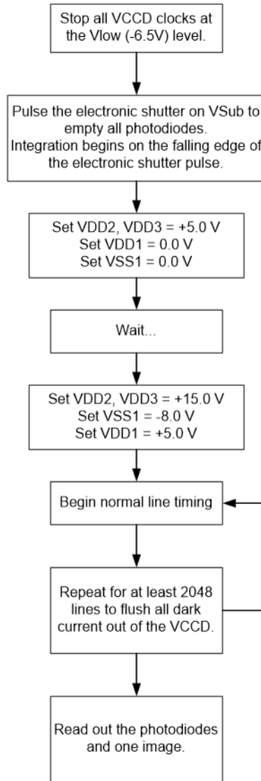
Figure 34. Timing Flow Chart for Long Integration Time
