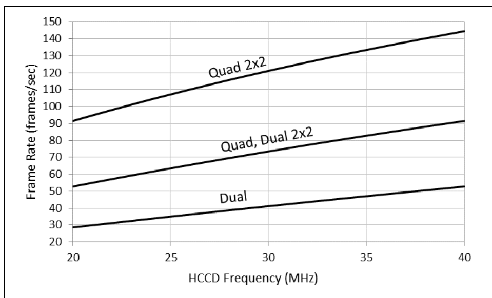
Figure 10. Frame Rates vs. Clock Frequency
