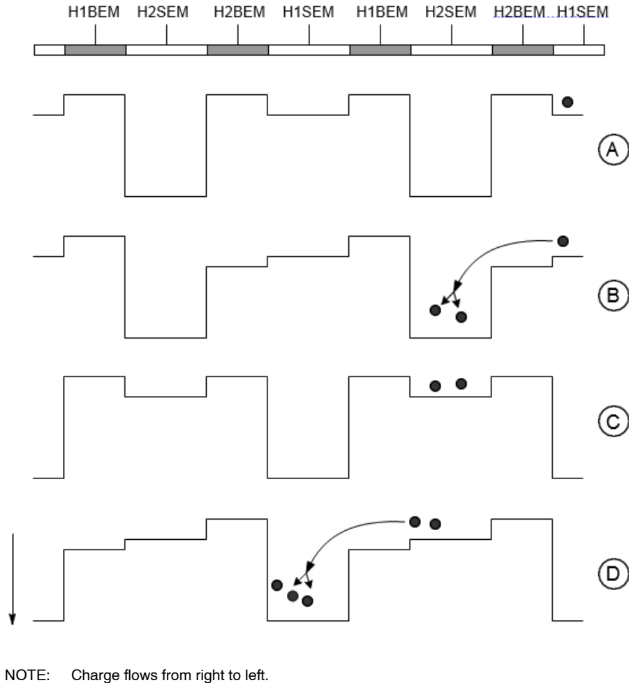
Figure 21. The Charge Multiplication Process
