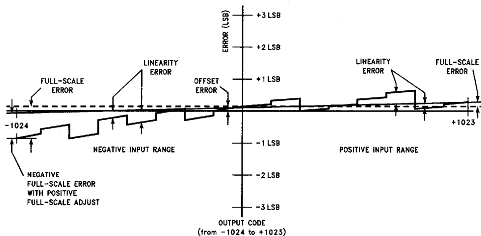
FIGURE 1B. Simplified Error Curve vs Output Code
