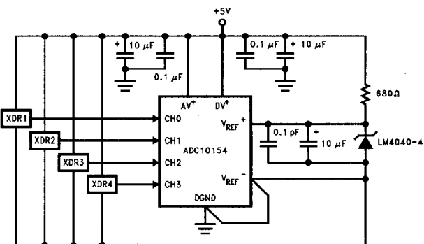
b. Absolute Using a 4.096V Span
