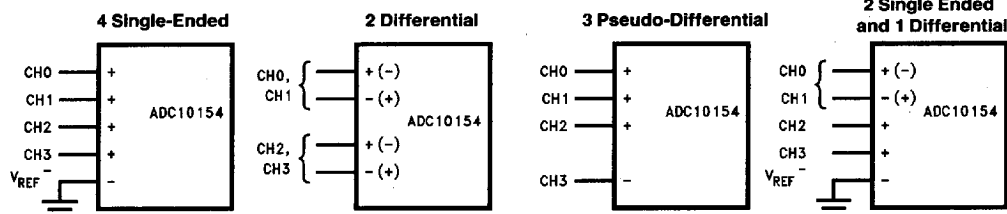
FIGURE 3. Analog Input Multiplexer Options
