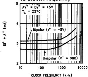
Total Positive Power Supply Current ( DI^+ + AI^+ ) vs Clock Frequency
