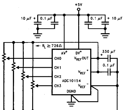
a. Ratiometric Using the Internal Reference
