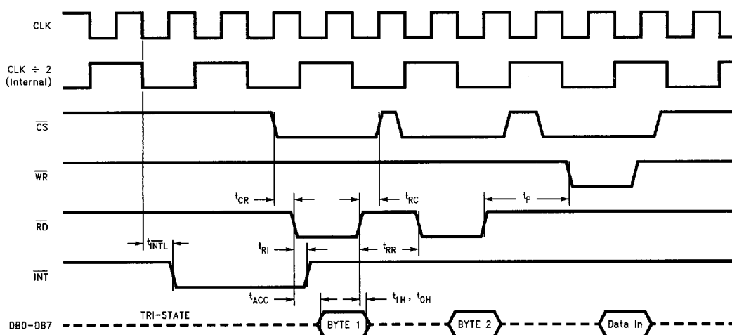
DIAGRAM 3. Reading the Conversion Result
