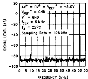
Spectral Response with 50 kHz Sine Wave
