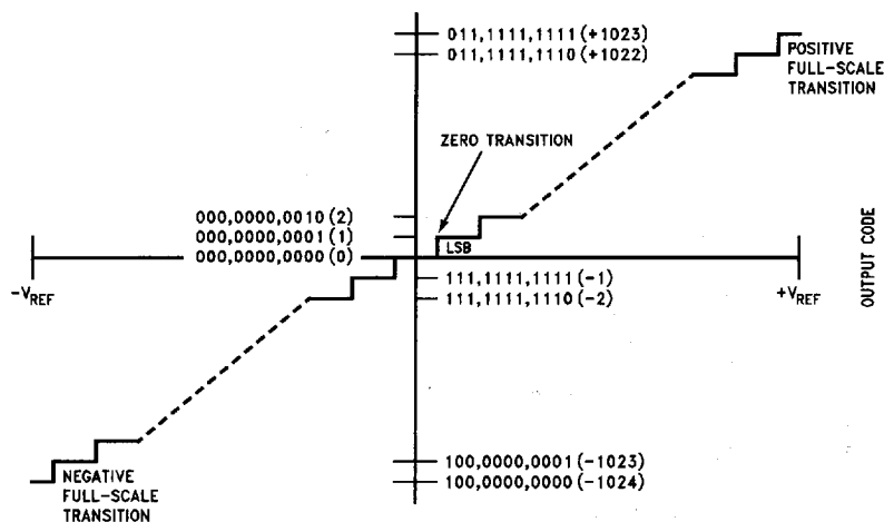
FIGURE 1A. Transfer Characteristic
