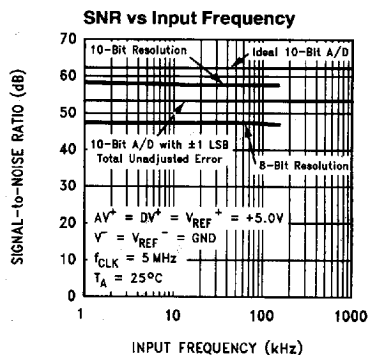
FIGURE 6. ADC10154/ADC10158 Signal-to-Noise Ratio vs Input Frequency
