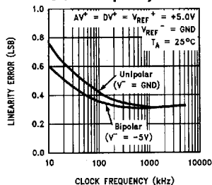
Linearity Error vs Clock Frequency
