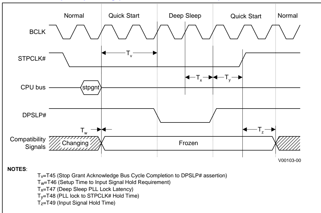
Figure 18. Quick Start/Deep Sleep Timing (DPSP# Assertion Method)
