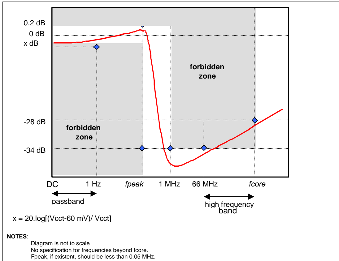
Figure 30. PLL Filter Specifications
