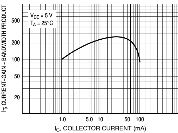
Figure 18. Current-Gain - Bandwidth Product
