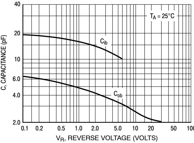
Figure 17. Capacitance
