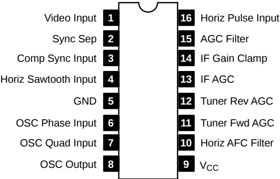
Pin Connection Diagram
