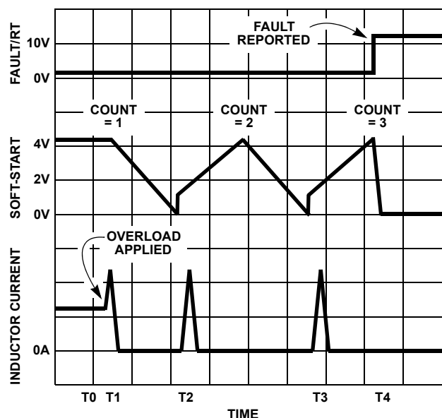
FIGURE 5. OVER-CURRENT OPERATION
