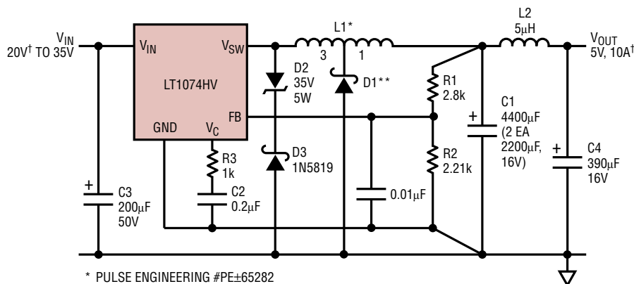
Tapped-Inductor Buck Converter
