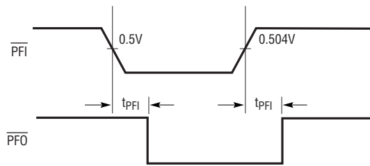
Figure 7. Power Fail Comparator Timing
