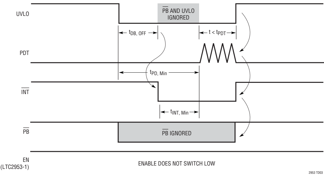
Figure 3. UVLO Interrupt Pulse: UVLO Low for t_{DB, OFF} < t < (t_{PD, Min} + t_{PDT}) (Enable Remains Active)
