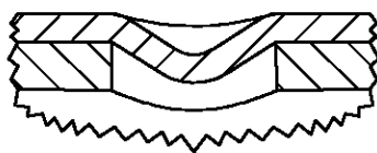
SECTION C-C SCALE 20:1
