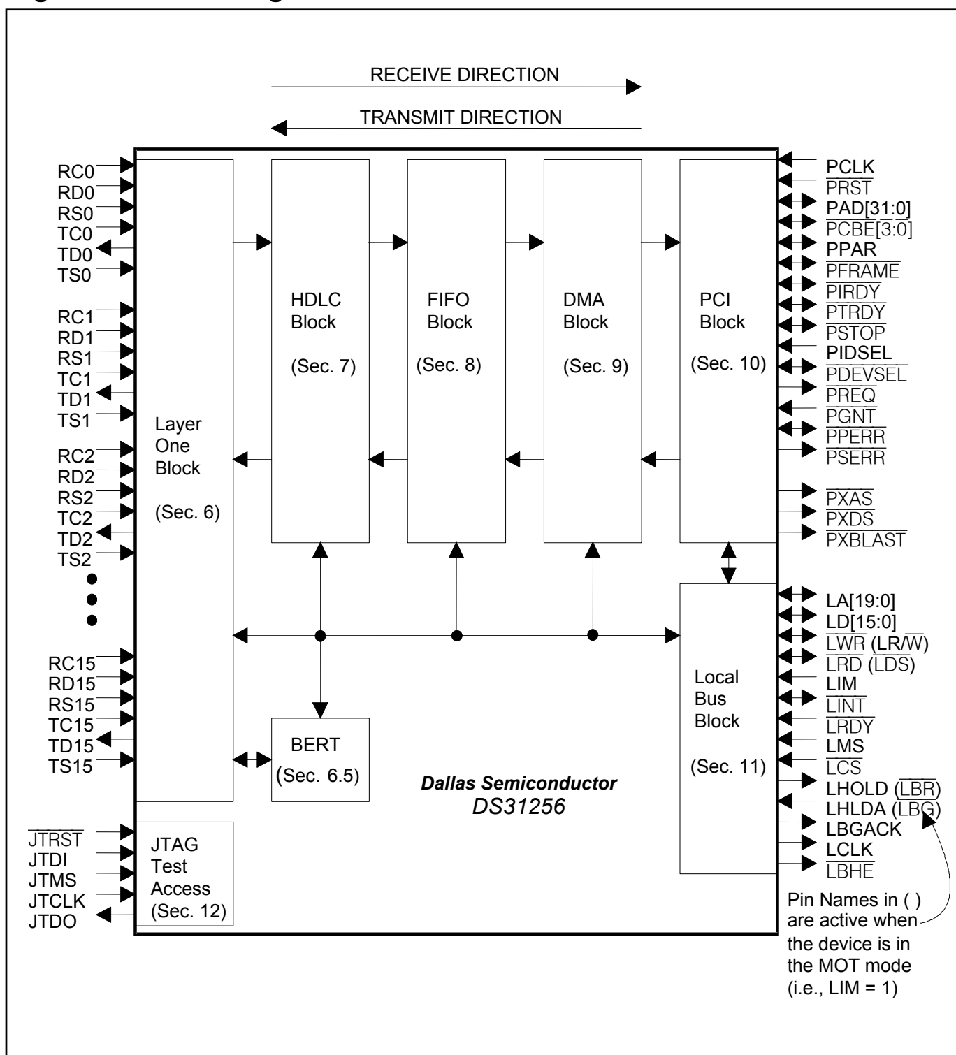
Figure 2-1. Block Diagram
