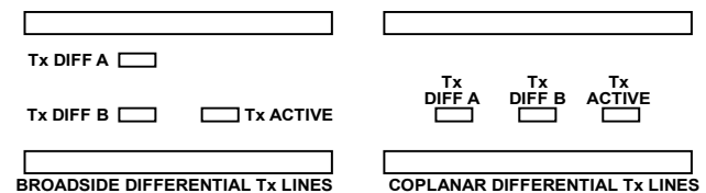
Figure 125. Broadside vs. Coplanar Differential Stripline Routing Techniques
