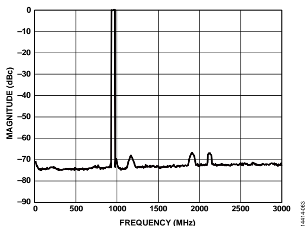
Figure 68. Eight Carriers at 950 MHz Output
