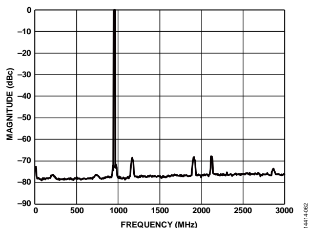
Figure 67. Four Carriers at 950 MHz Output
