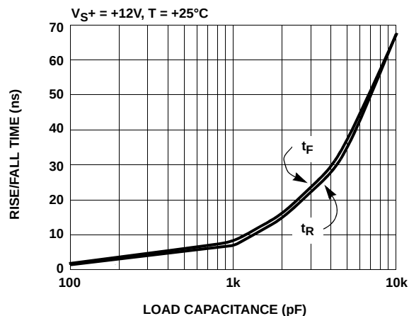
FIGURE 8. RISE/FALL TIME vs LOAD CAPACITANCE
