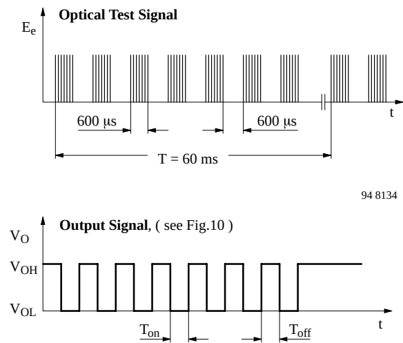
Figure 8. Output Function
