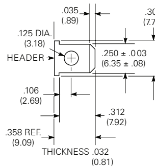
6.35mm (.250") Quick Connect/Solder
