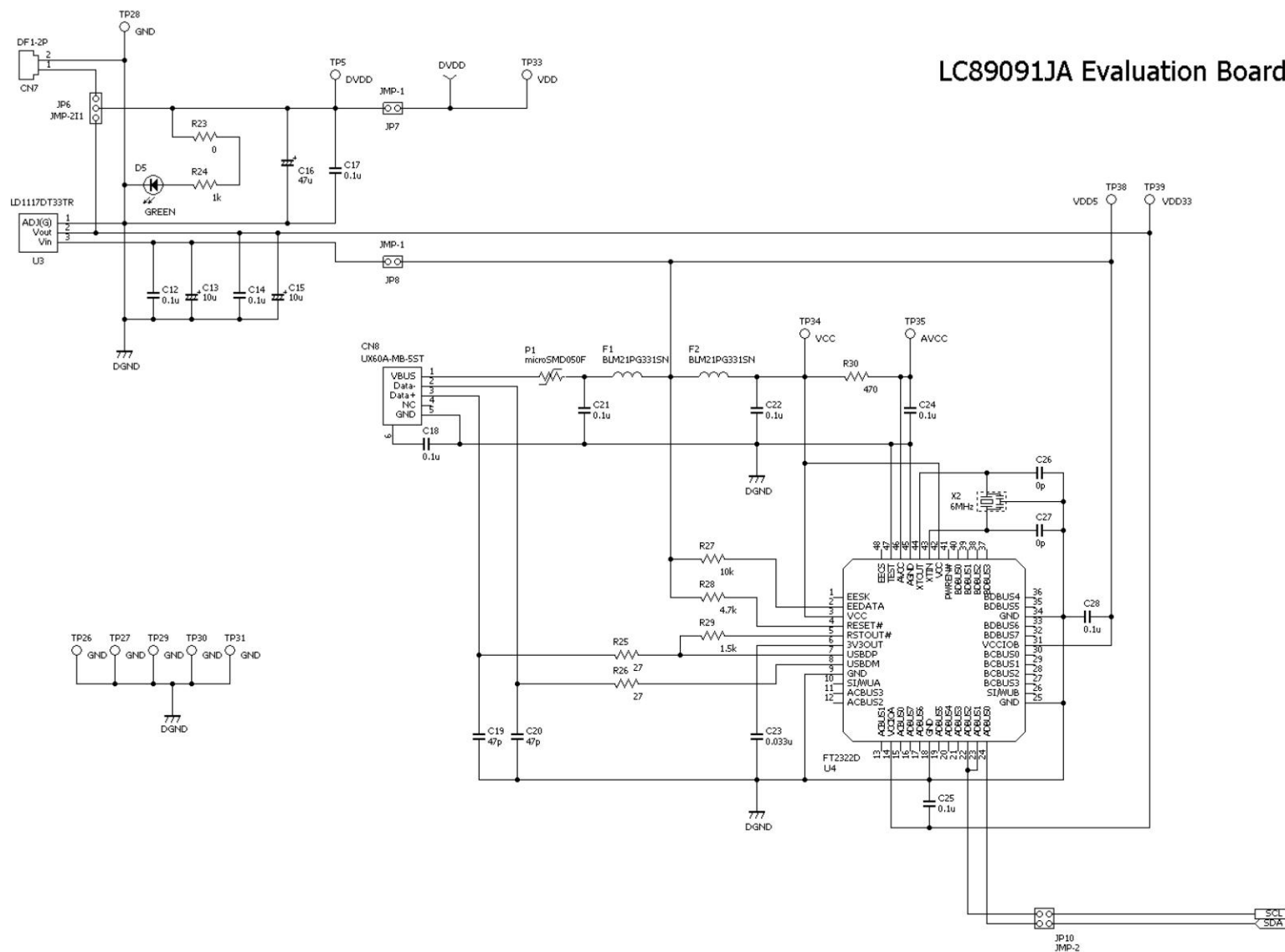
USB Microcontroller Peripheral Circuitry
