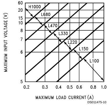
FIGURE 3. LM2575(HV)-3.3
