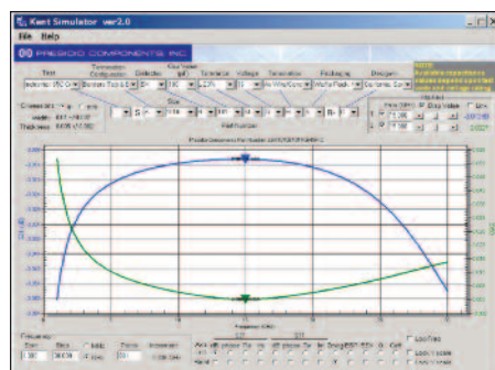
Fig. 5. Modeled S21 and Z/50 of part LSA1010B101MGH5R-, Class II Dielectric
