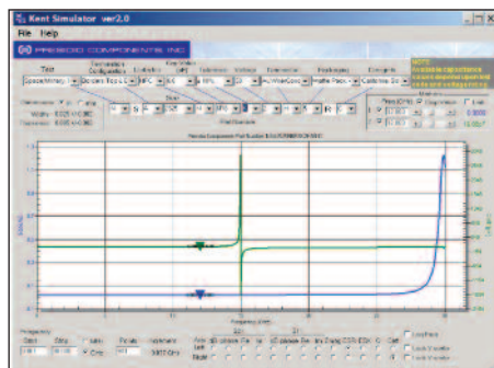
Fig. 4. Modeled ESR/50 and Ceff of part NSA2525N6R8K2H5R-
