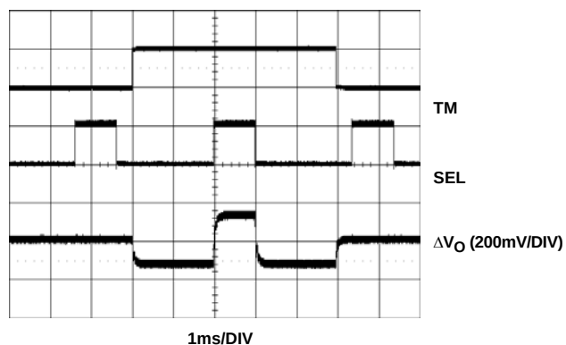
FIGURE 16. VOLTAGE MARGINING
