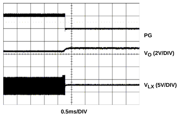
FIGURE 17. OVER-VOLTAGE SHUT-DOWN
