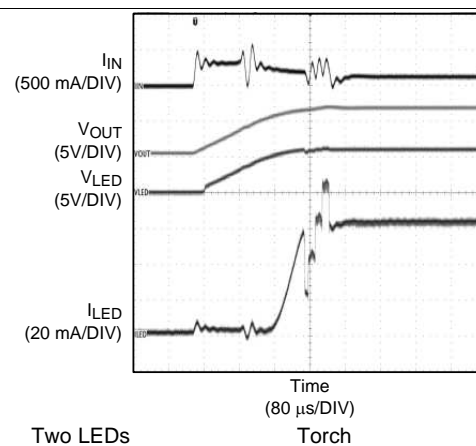
Figure 30. Diode Detect
