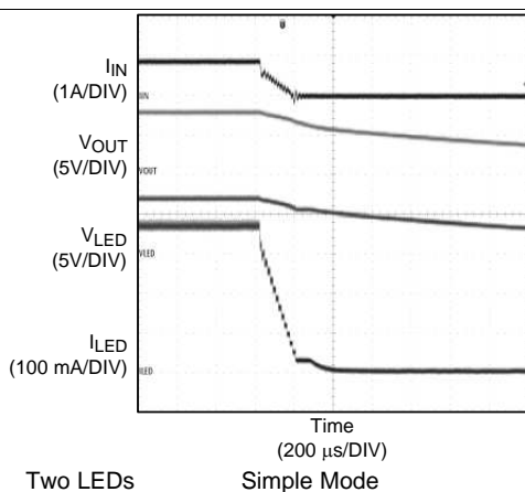
Figure 29. Ramp-Down
