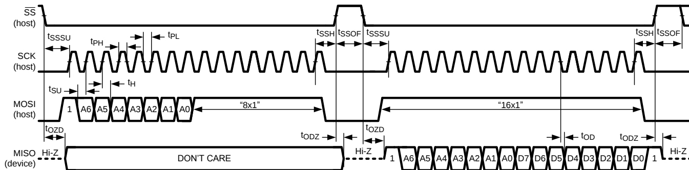
Figure 5. SPI Read
