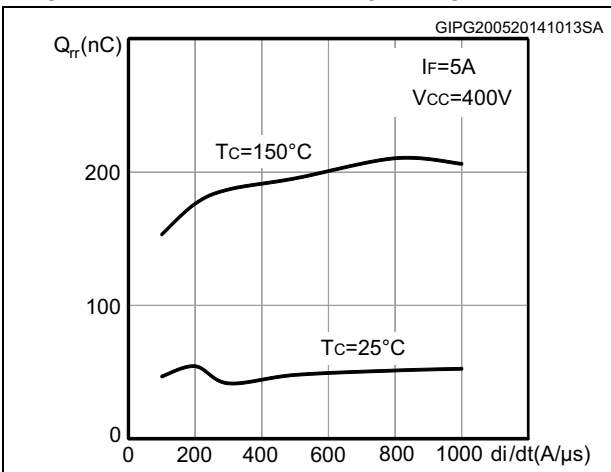
Figure 24. Reverse recovery charges vs. di/dt
