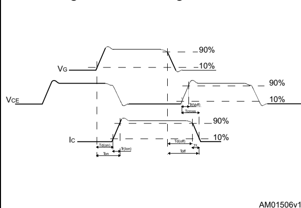
Figure 29. Switching waveform
