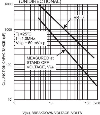
FIG.5- TYPICAL JUNCTION CAPACITANCE (UNIDIRECTIONAL)
