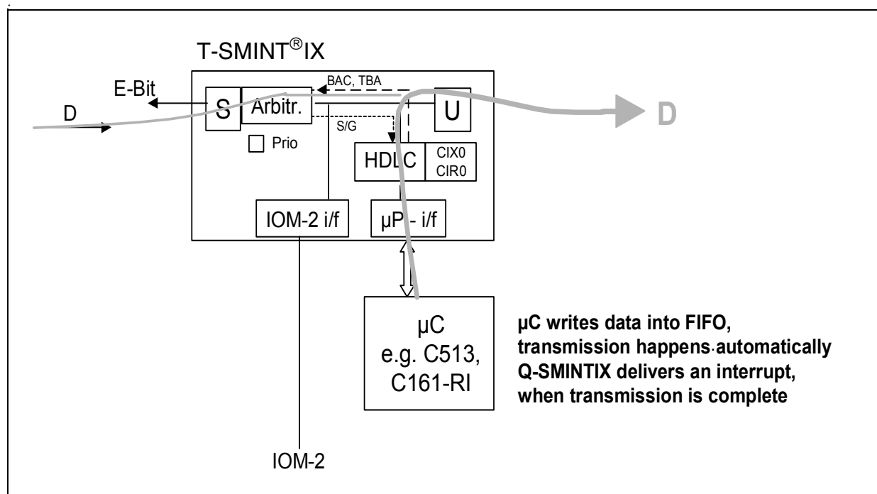
Figure 26 D-Channel Arbitration: \mu C has no HDLC and no Direct Access to TIC Bus
