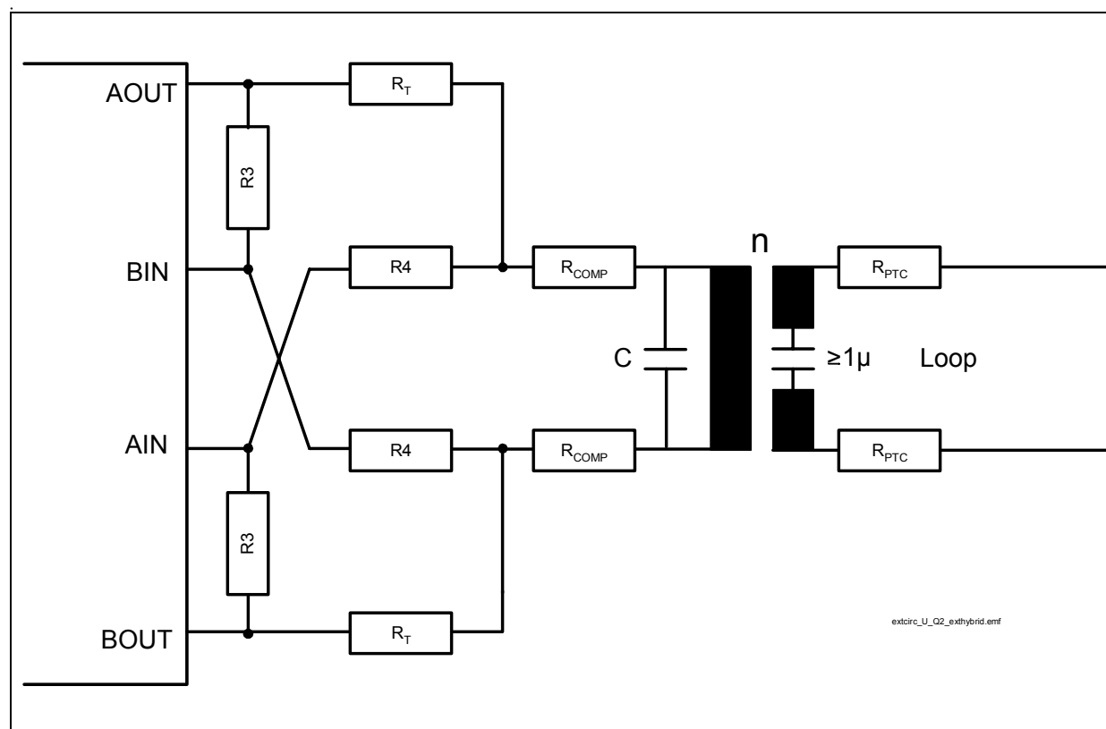
Figure 88 External Circuitry Q- and T-SMINT ® IX
