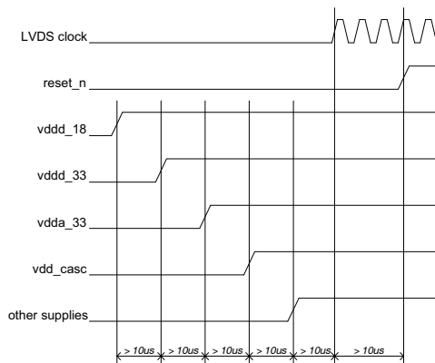
Figure 17. Power-up Procedure
