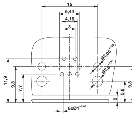
Drilling diagram
