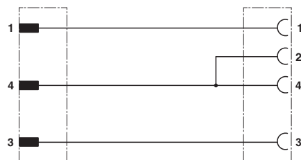
Circuit diagram
