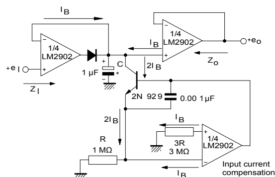
Figure 30. Low drift peak detector
