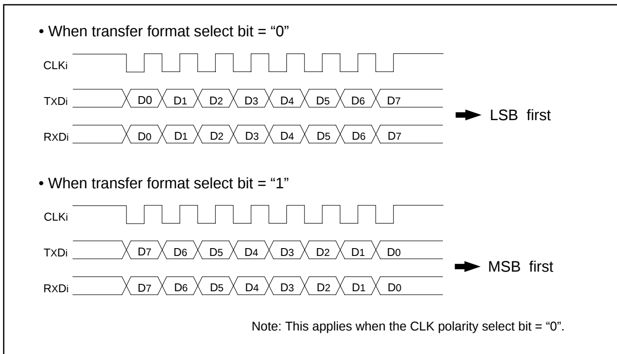
Figure 1.19.12. Transfer format
