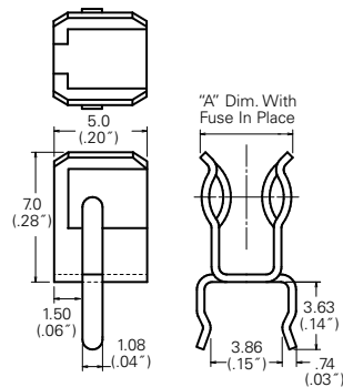
111 501 / 111 506 Device Dimensions
