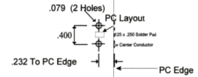
V-Bite PCB
