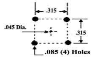
PCB Layout 864B Series
