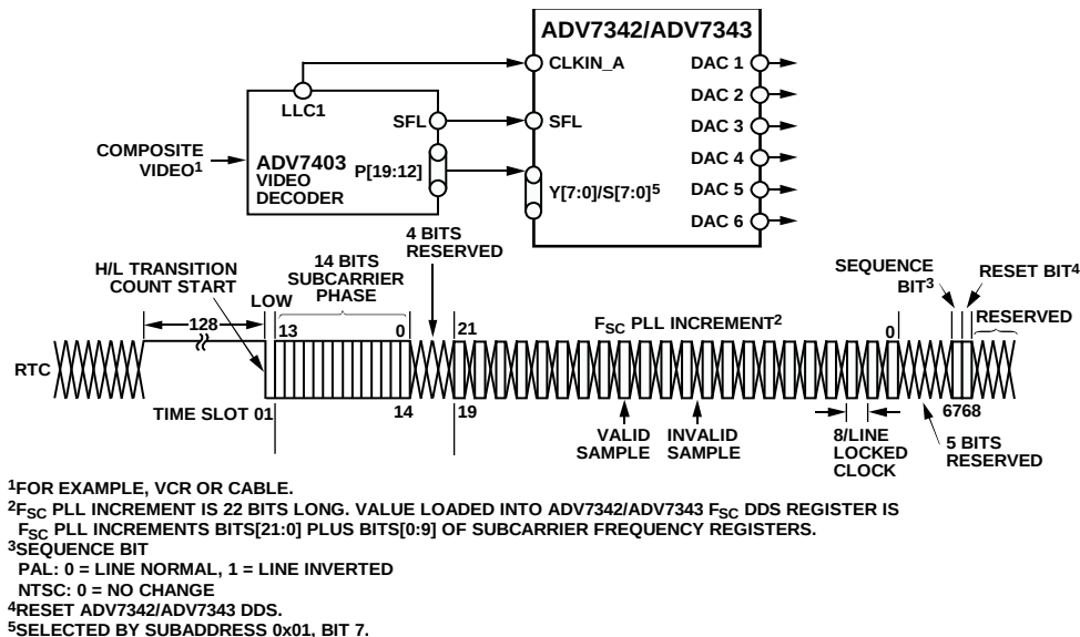
Figure 59. SD Subcarrier Frequency Lock Timing and Connections Diagram (Subaddress 0x84, Bits [2:1] = 11)
