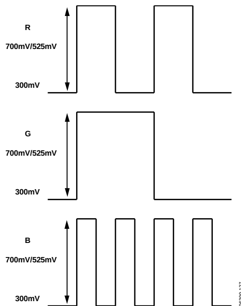
Figure 125. HD RGB Output Levels—RGB Sync Disabled
