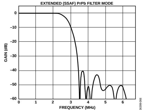
Figure 62. PrPb SSAF Filter
