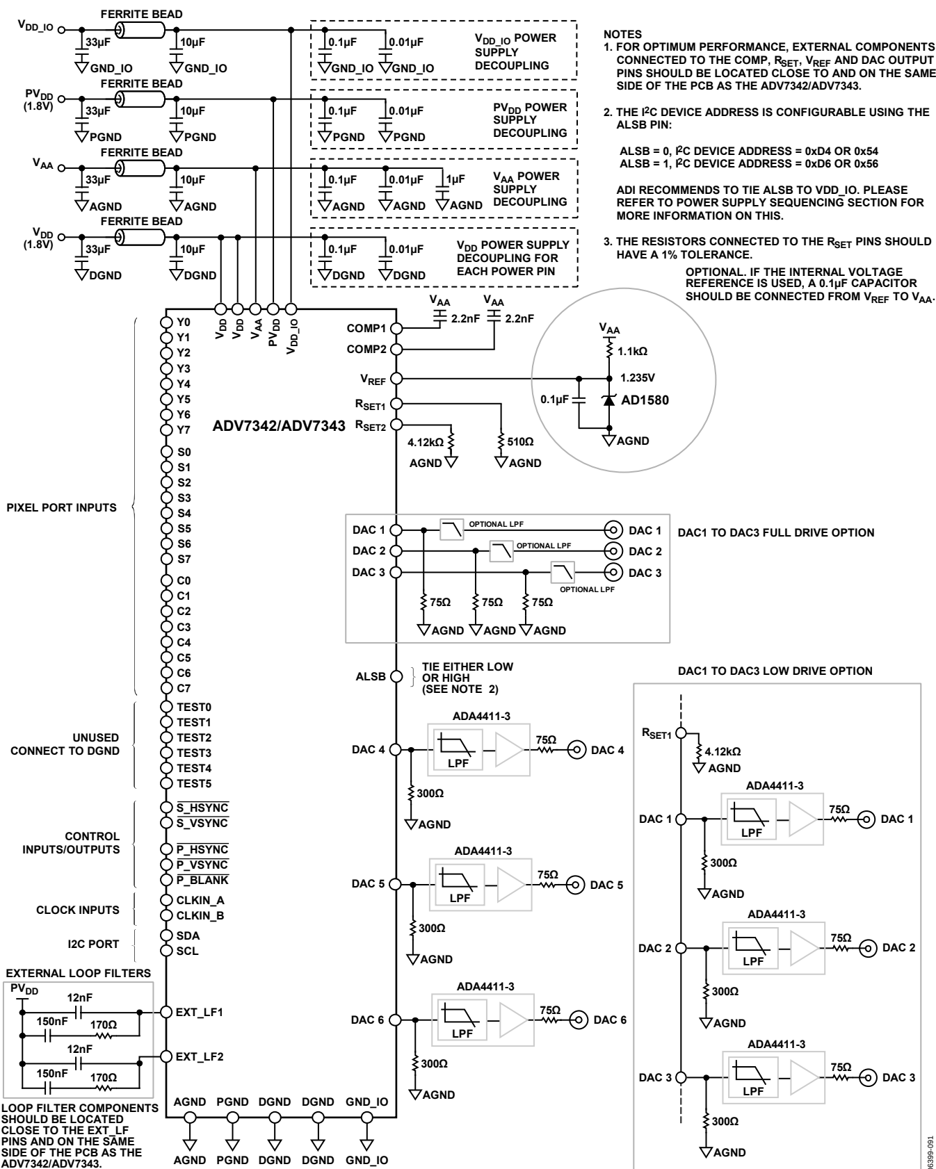
Figure 89. ADV7342/ADV7343 Typical Application Circuit
