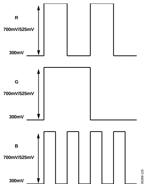
Figure 123. SD/ED RGB Output Levels—RGB Sync Disabled
