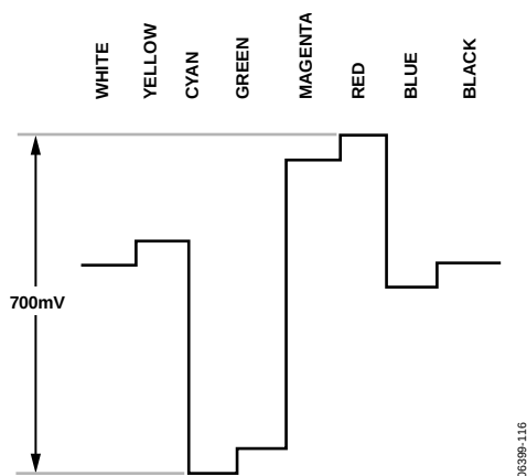
Figure 114. Pr Levels—NTSC
