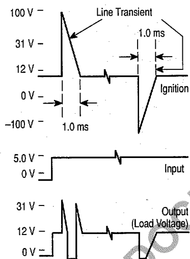
Figure 2. Timing Diagram
