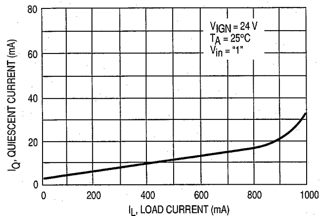
Figure 5. Quiescent Current versus Load Current
