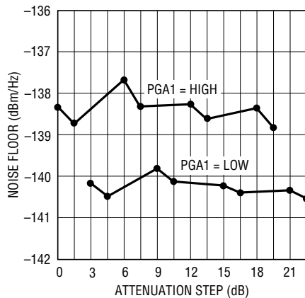
Output Noise Floor vs Attenuation Step, Freq = 100MHz, R_{OUT} = 200\Omega
