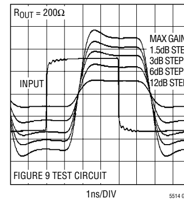
Pulse Response vs Attenuation, LT5514 Levels are: V_{IN} = 66mV_{P-P} , V_{OUT} = 4V_{P-P} at Max Gain
