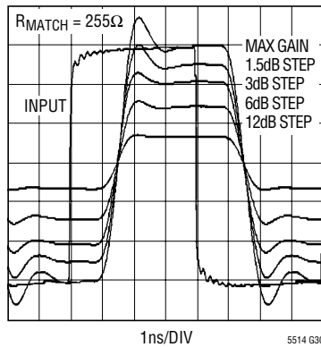
Pulse Response vs Attenuation, LT5514 Levels are: V_{IN} = 66mV_{P-P} , V_{OUT} = 2V_{P-P} at Max Gain
