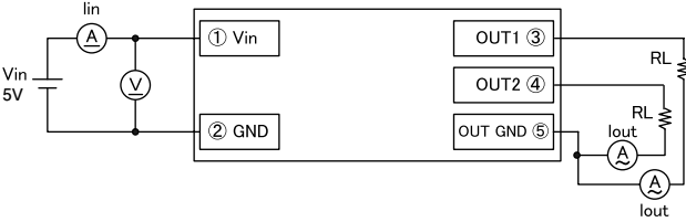
CONNECTION D
