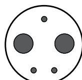
23-24320 2 Size 4 Contacts 3 Size 20 Contacts
