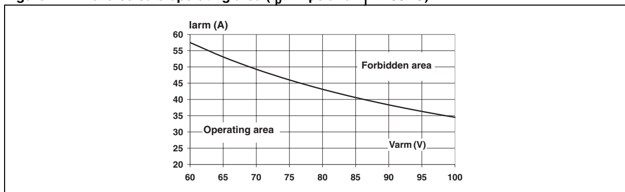
Figure 12. Reverse safe operating area ( t_p < 1 \mu s and T_j < 150^\circ C )
