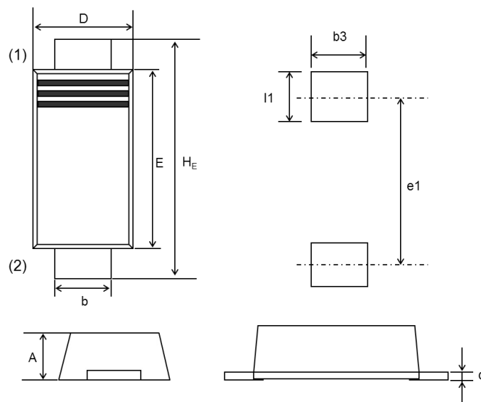
SOD-123FL, [SC-109B], (PMDU)
